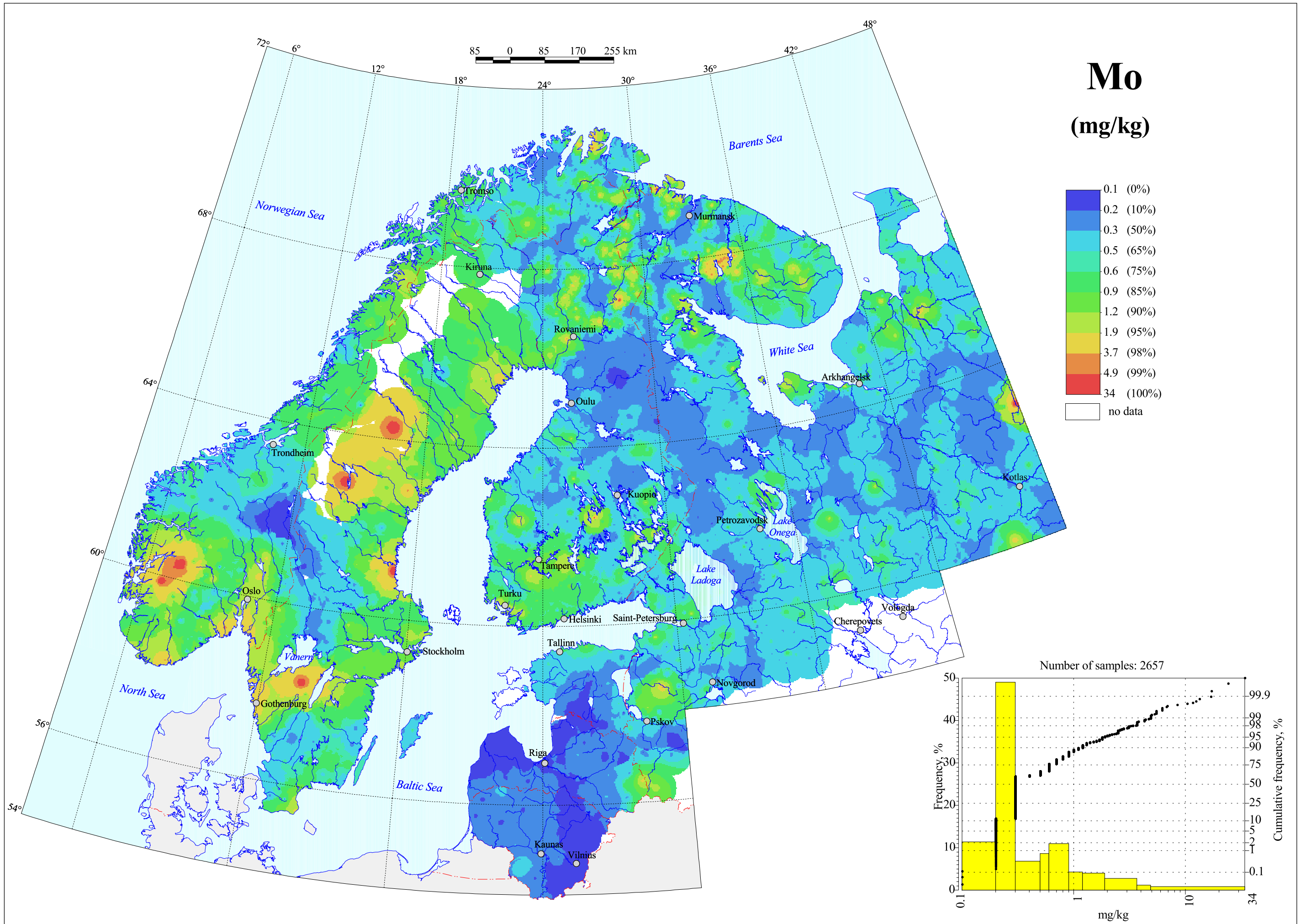
Molybdenum in C-horizon, Grain Size <2 mm, Total Content
